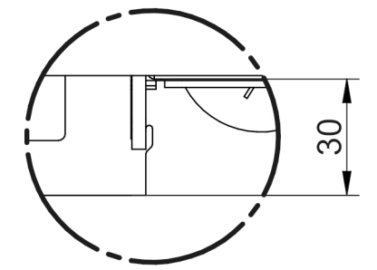
DETAIL A 1:2
