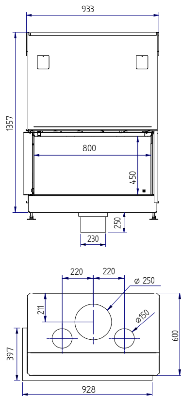
Plan = Luna 900 CL
