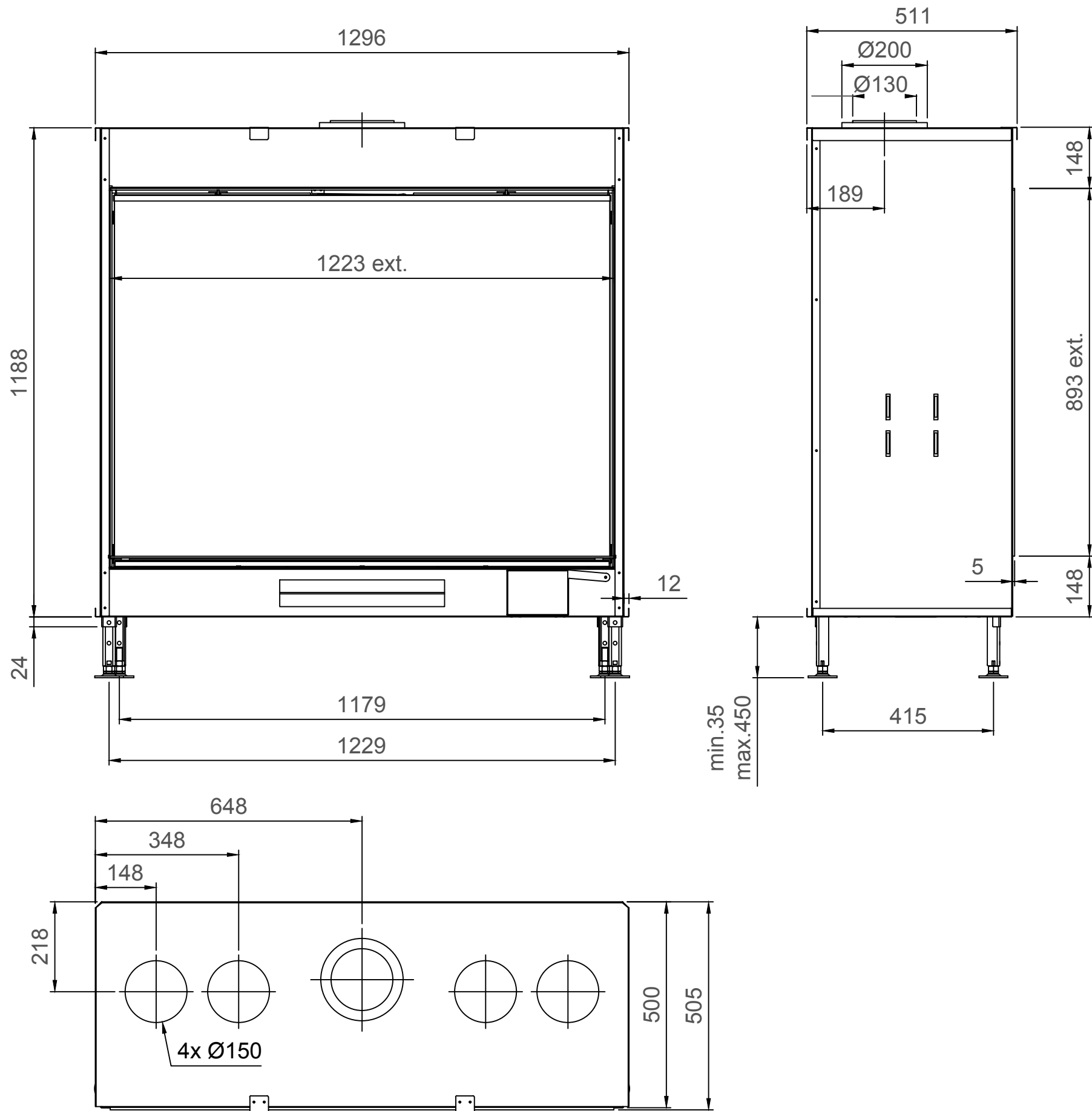
True Vision 1300V - Type 1 - Coverframe
